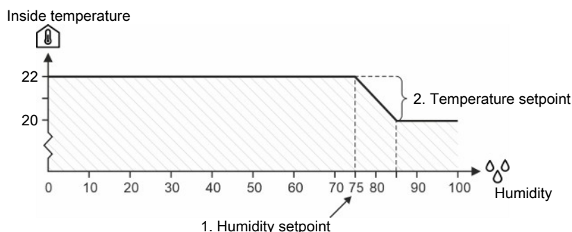
Figure 6: Humidity control with temperature reduction
