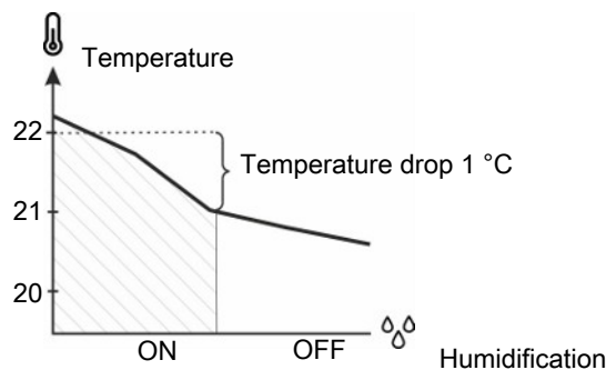
Figure 5: Decreasing temperature: Humidification will be disconnected if the inside temperature is 1° C below Temperature setpoint. Humidification could otherwise make the inside temperature drop further.
