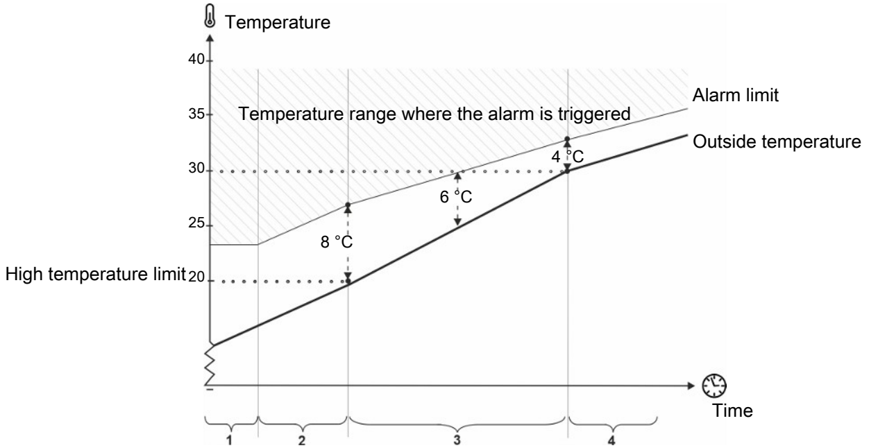
Figure 9: Summer temperature at 20°C and 30°C outside
