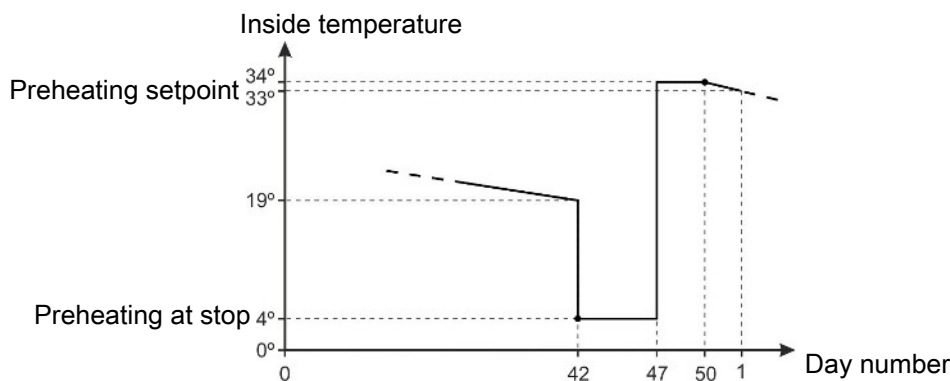
Figure 8: Example of setting of preheating.
