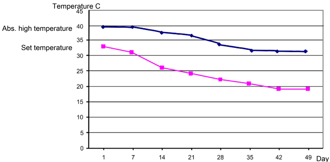
Figure 10: Example of Absolute high temperature alarm.
