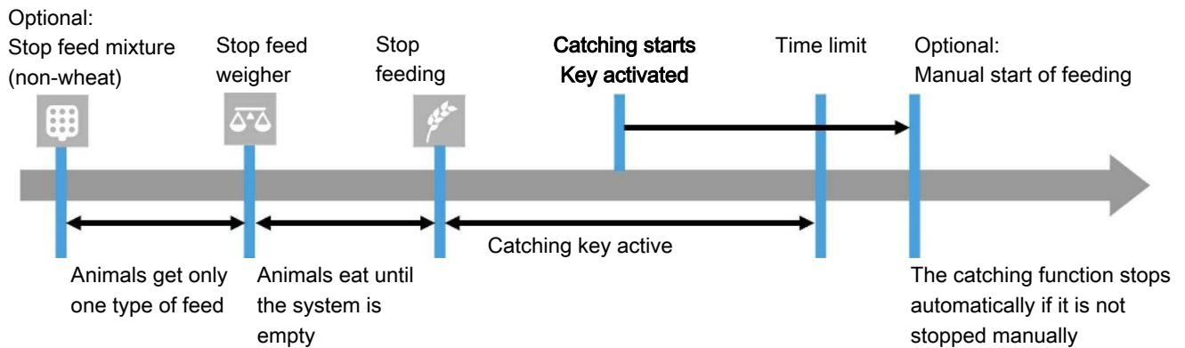
Figure 7: The sequence when stopping the feed system during catching
